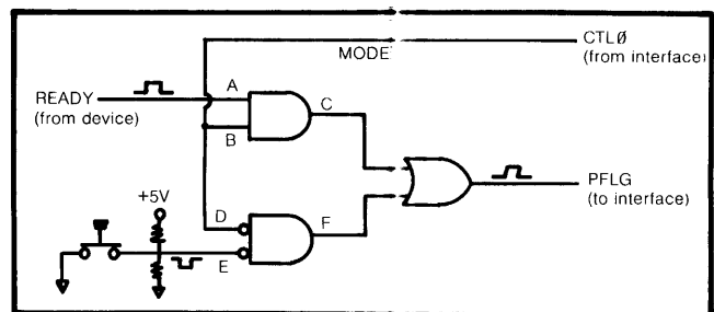
Figure I-16: An Example Use of Logic Elements
