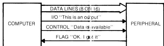
Figure I-8. Data Output Handshake
